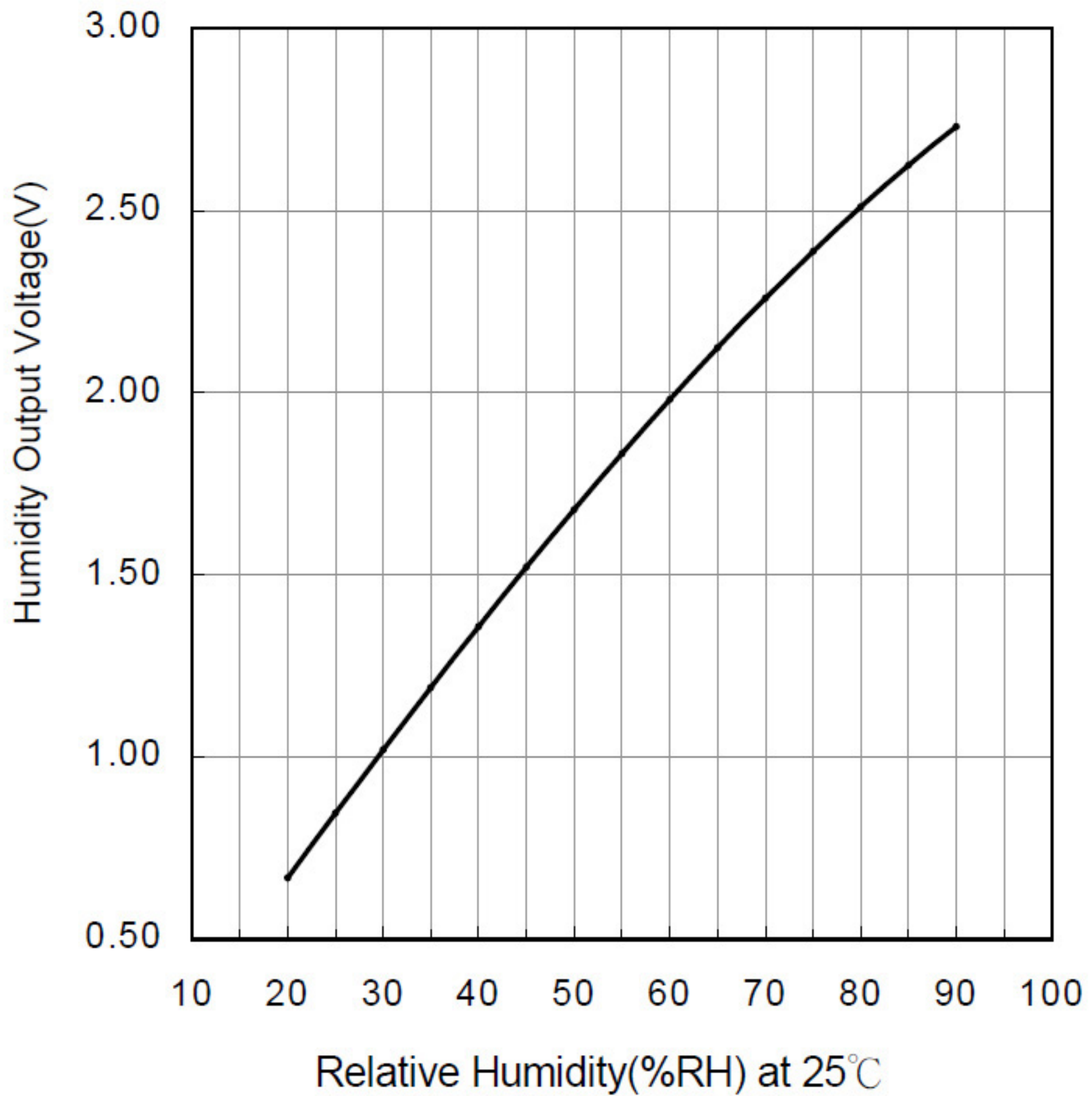
HMZ-333A1 Humidity Output 0~3.3V characteristics
